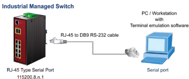
Figure 3: Console connectivity
